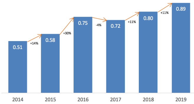
EPS (PHP/SH)
