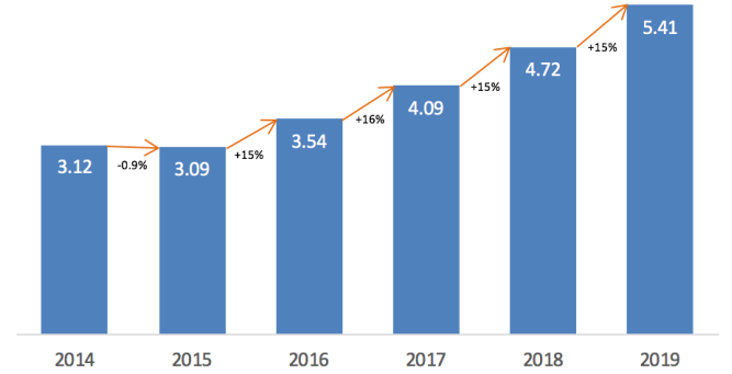
BVPS (PHP/SH)
