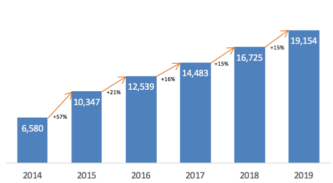
BVPS (PHP/SH)
